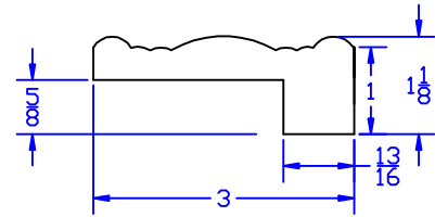
(DM #8) Z-Frame
