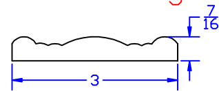
(S-28) Casing
