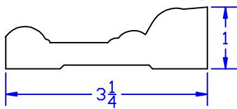
#338 MDF Casing
