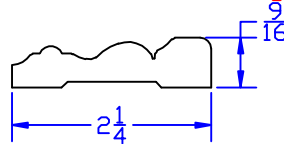
#314 MDF Casing
