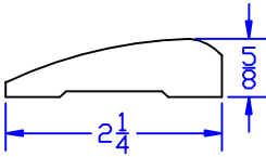
#326 MDF Casing
