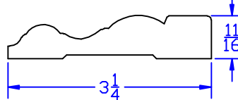
#388 MDF Casing
