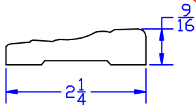
#366 MDF Casing
