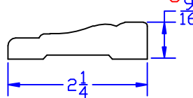
#356 MDF Casing
