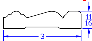
#312 MDF Casing
