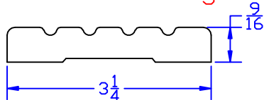
#396 MDF Casing
