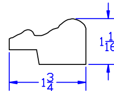
51 Panel Cap
