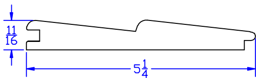
70114 T&G Lap Siding
